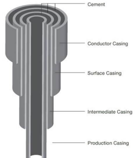
Figure 1: Typical Well Casing Set Up
